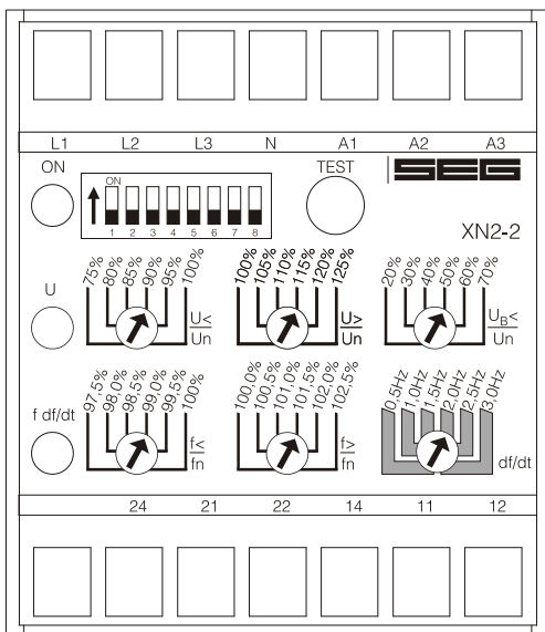
Figure 4.2: Front plate XN2-2
