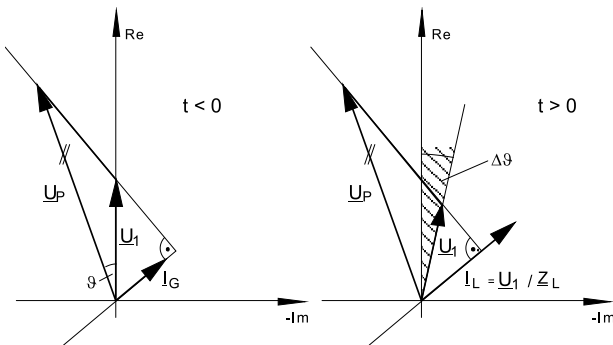
Figure 3.2: Vector diagram rotor displacement angle and voltage vector
