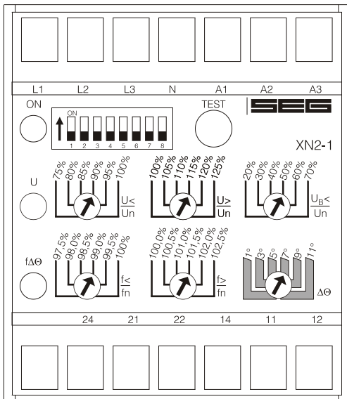
Figure 4.1: Front plate XN2-1
